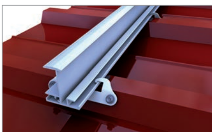
Insertion rail on EPDM with trapezoidal clamp
