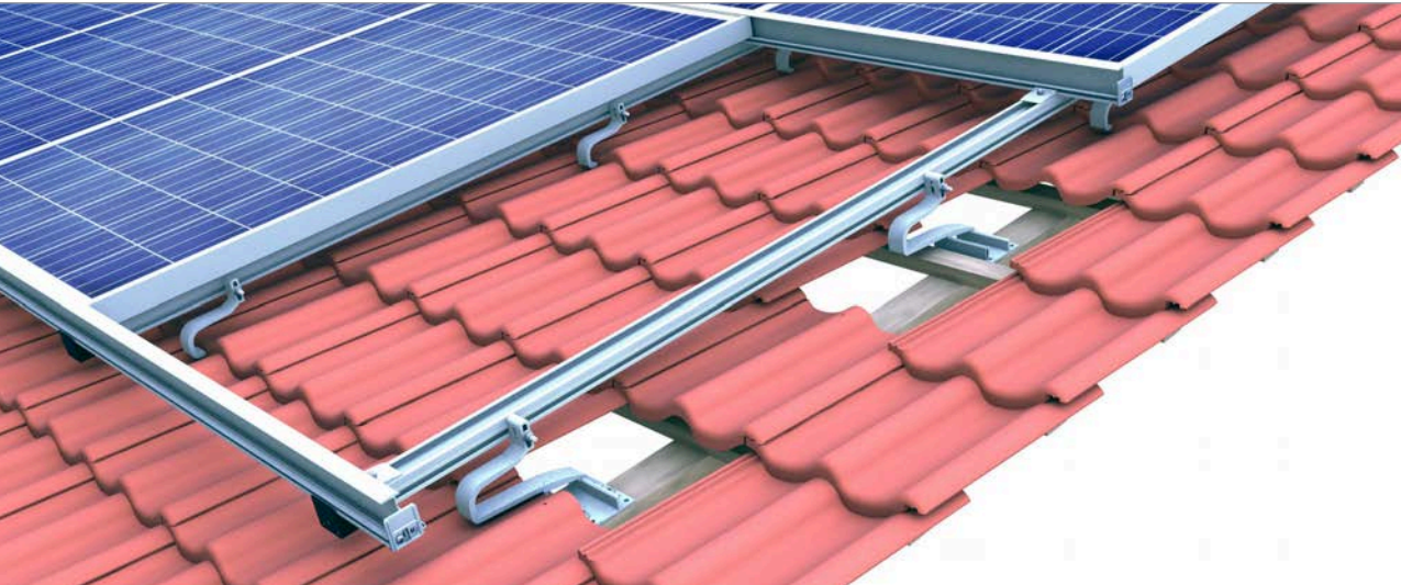
novotegra side-fix – insertion system with modules installed in portrait
