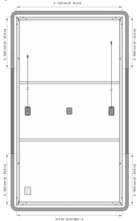
Fig. 23: REC Alpha 72 Series MLPE device installation zones
