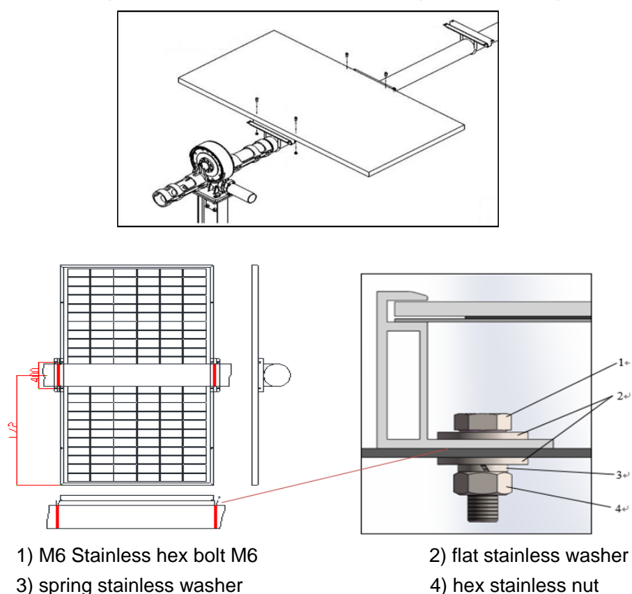
Fig 2. PV module installed with Single-axis Tracing System
