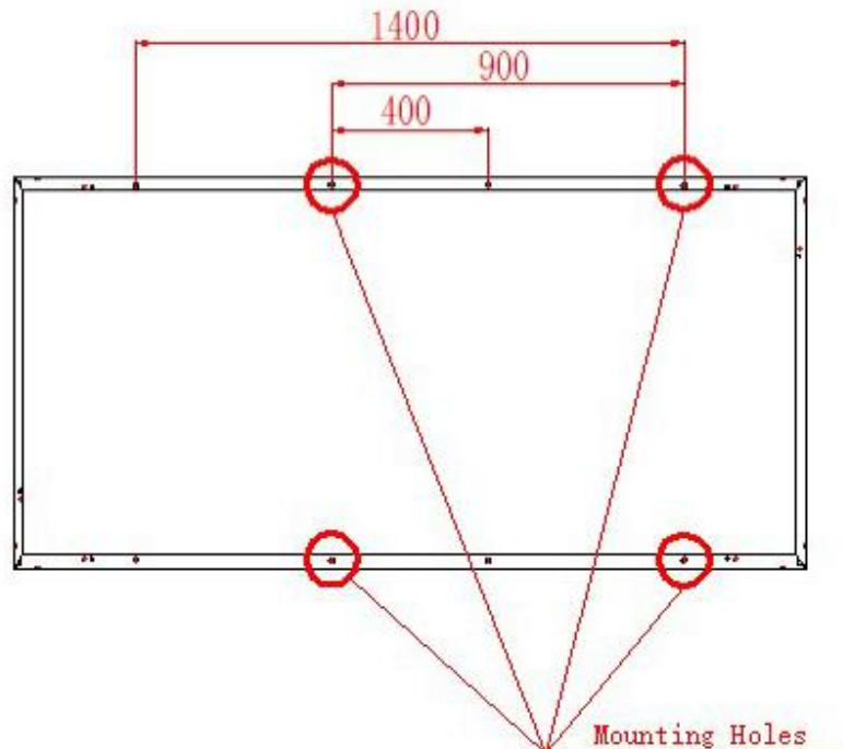
Figure 3: Mounting holes schematic of the single module for the 2V installation method
