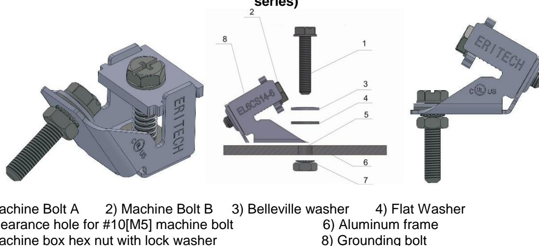
Figure 6. ERICO grounding bolt # EL6CS14-6 (NOT applicable for the TRINAMOUNT module series)
