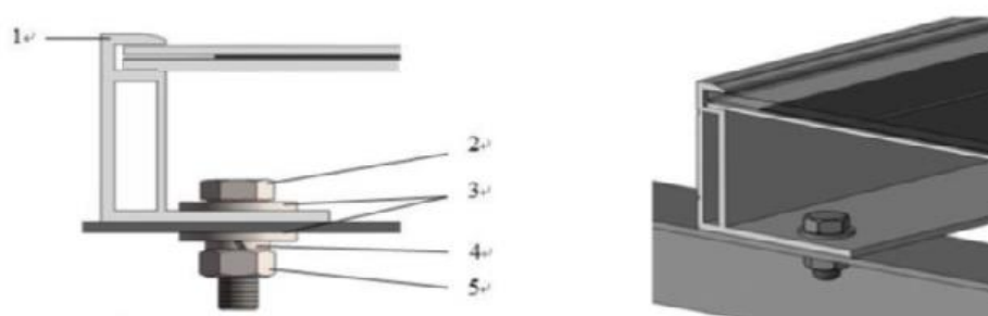
Figure.1 Duomax serial module with frame
