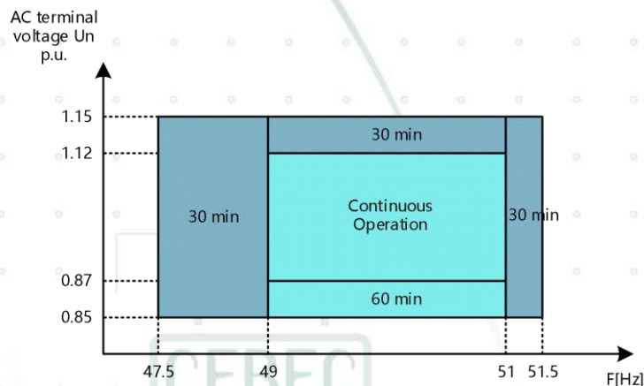
Figure 3 Quasi-stationary operation range for MODEL SOFAR 50KTLX-G3
