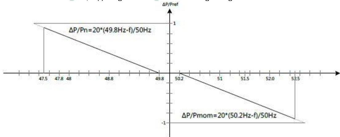
Figure 6 MODEL SOFAR 50KTLX-G3 P(f)-diagram
