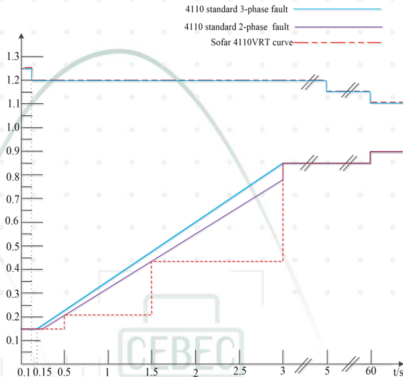
Figure 5 FRT limit curve for MODEL SOFAR 50KTLX-G3
