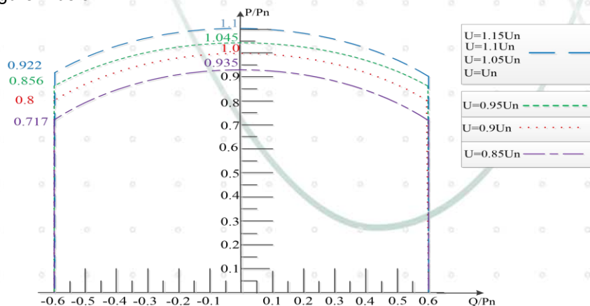
Figure 4 Voltage-dependent PQ diagram for MODEL SOFAR 50KTLX-G3
